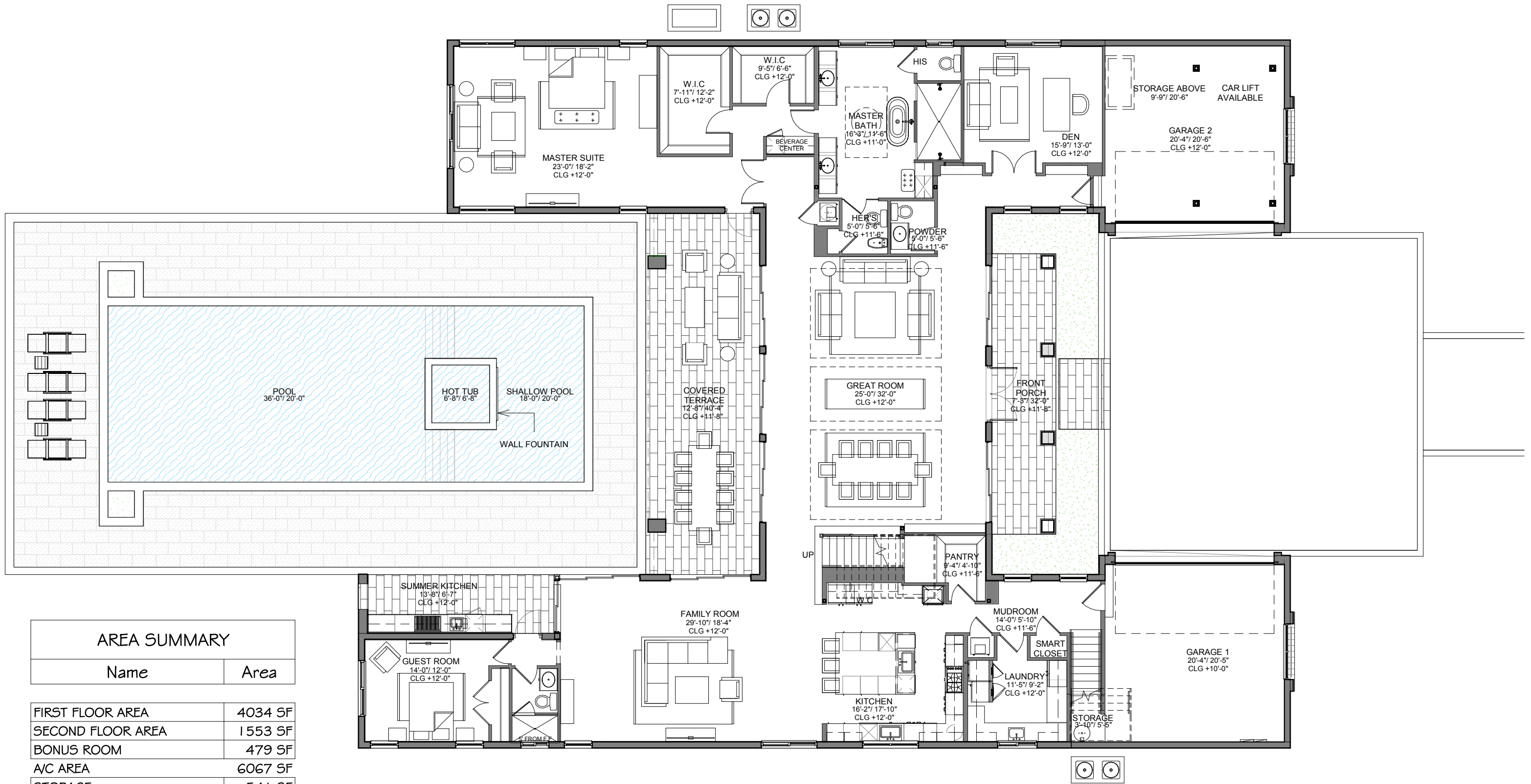
FIRST FLOOR PLAN 3/32" = 1'-0"
