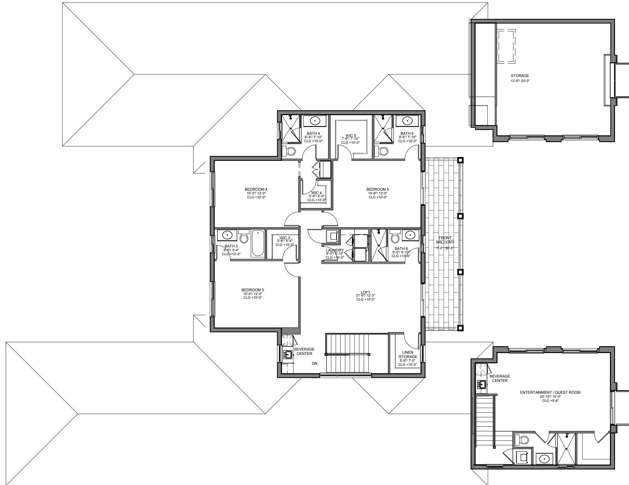
SECOND FLOOR PLAN 3/32" = 1'-0"
